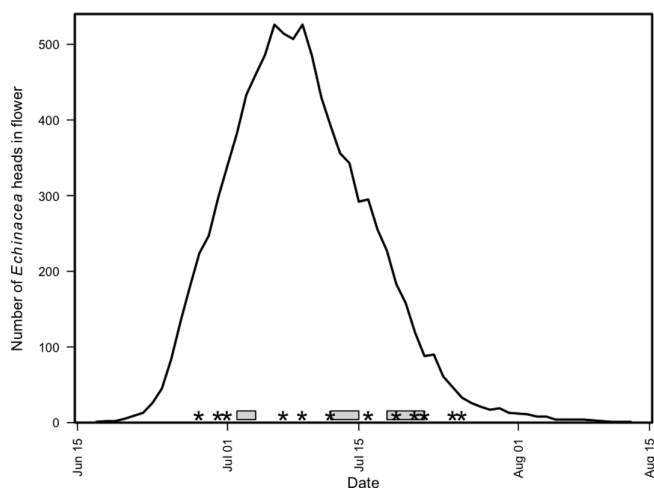
Figure 1. Total number of Echinacea flowering heads producing pollen per day at the eight remnant populations where we conducted pollinator observations (Table 1). The asterisks represent days when we conducted the pollinator observations. The gray bars indicate days when we collected pollinators from three of the sites (AA, EELR and LF) for the pollen load analysis.
